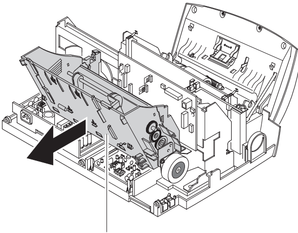
Automatic Sheet Feeder Assembly
